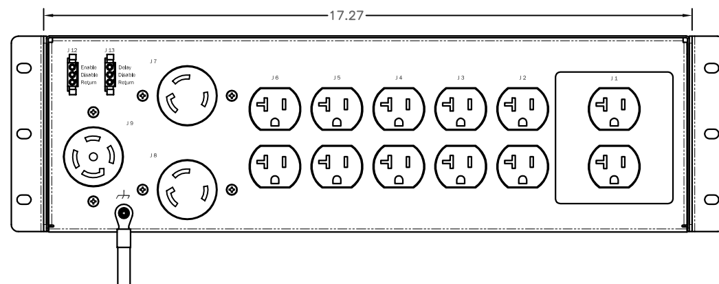
REAR VIEW
