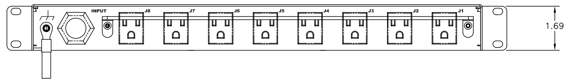
REAR VIEW
