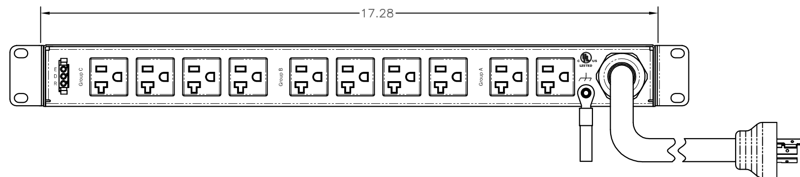
REAR VIEW
