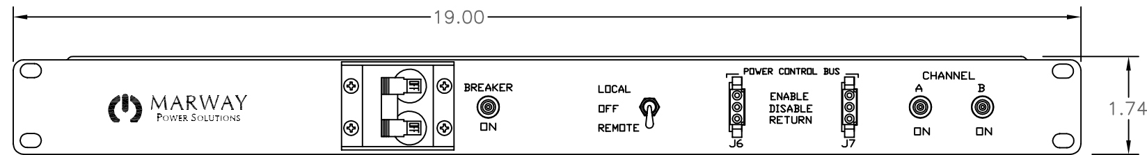
FRONT VIEW
