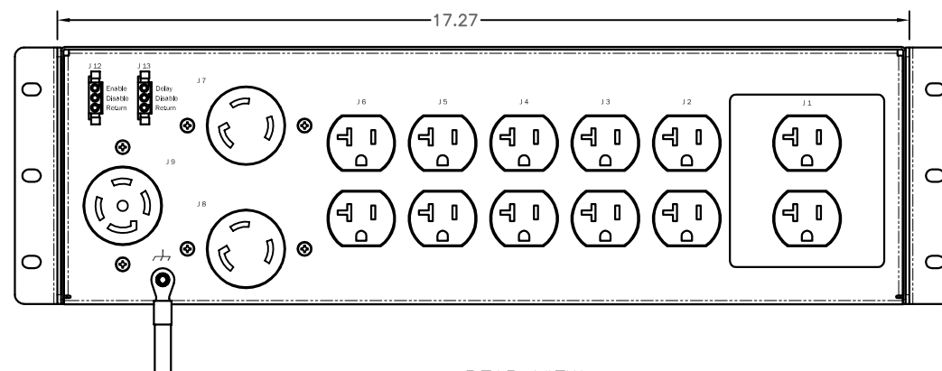
REAR VIEW
