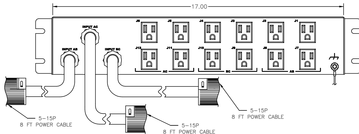
REAR VIEW
